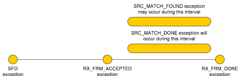
Figure 24 - Exceptions generated by source address matching
