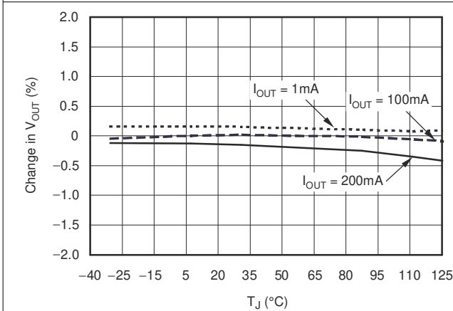
Figure 6-1. Load Regulation
