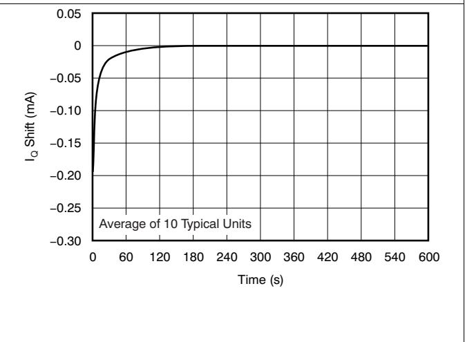
Figure 22. Normalized Quiescent Current vs Time
