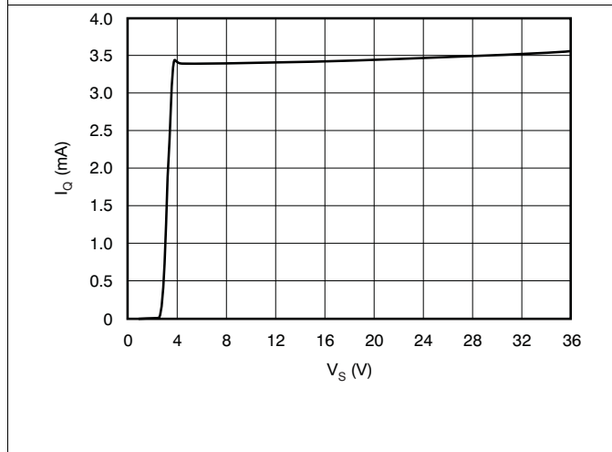
Figure 21. Quiescent Current vs Supply Voltage
