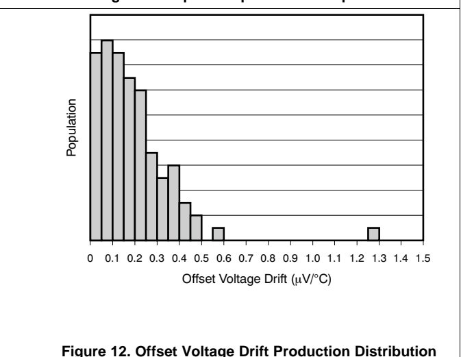
Figure 12. Offset Voltage Drift Production Distribution
