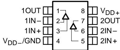
TLV2442 D OR JG PACKAGE (TOP VIEW)
