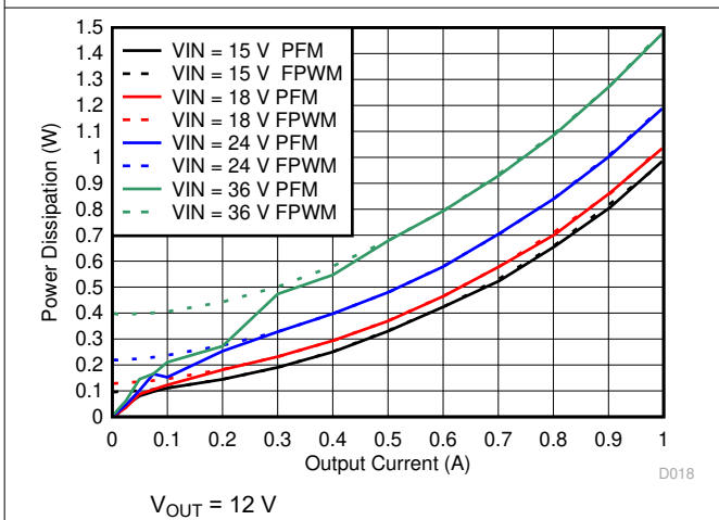
Figure 6-11. Power Dissipation
