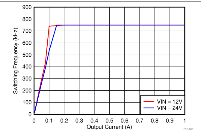
Figure 6-26. Auto PFM Mode Switching Frequency vs Output Current
