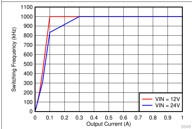
Figure 6-25. Auto PFM Mode Switching Frequency vs Output Current
