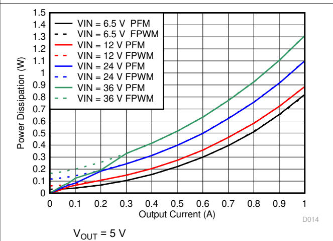
Figure 6-12. Power Dissipation
