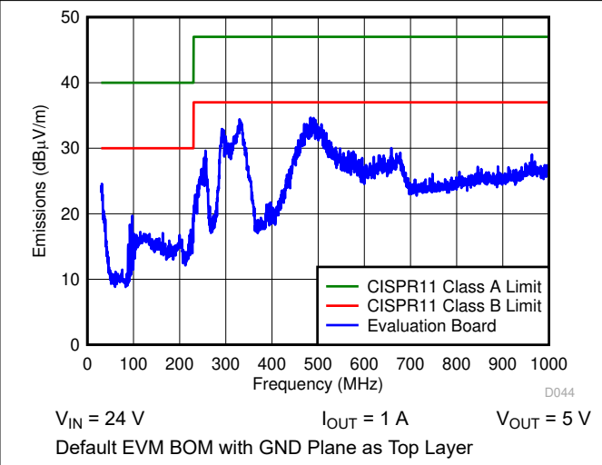
Figure 6-8. Radiated EMI
