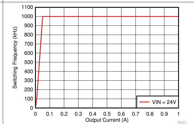
Figure 6-28. Auto PFM Mode Switching Frequency vs Output Current
