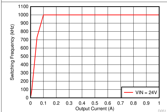
Figure 6-27. Auto PFM Mode Switching Frequency vs Output Current
