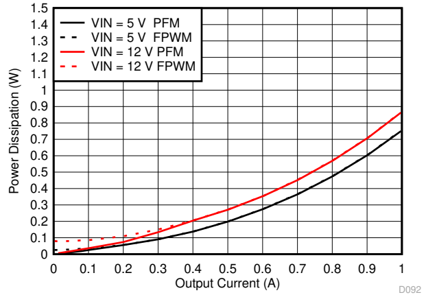
Figure 6-14. Power Dissipation
