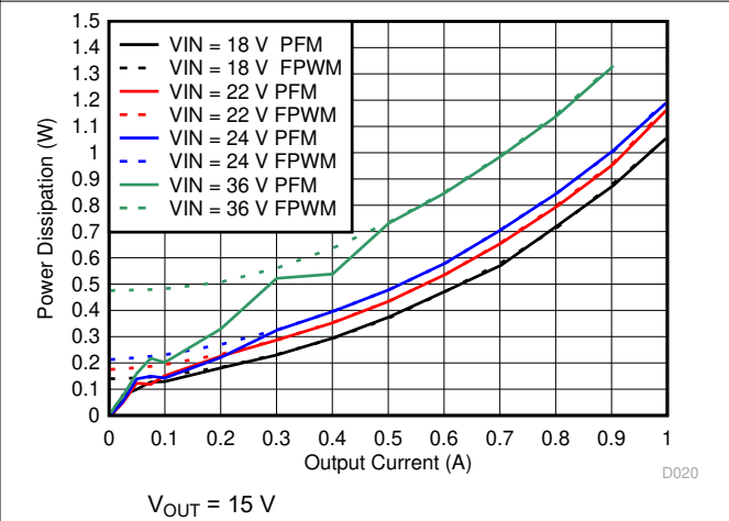
Figure 6-10. Power Dissipation
