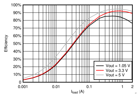
TPS562207 Efficiency
