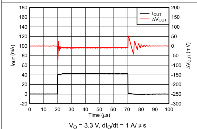
图 8-8. Load Transient Behavior for New Chip
