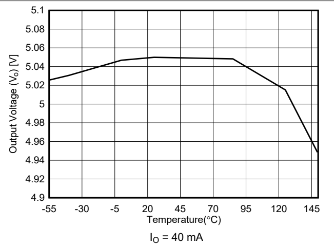
图 6-2. V_O vs Temperature for New Chip
