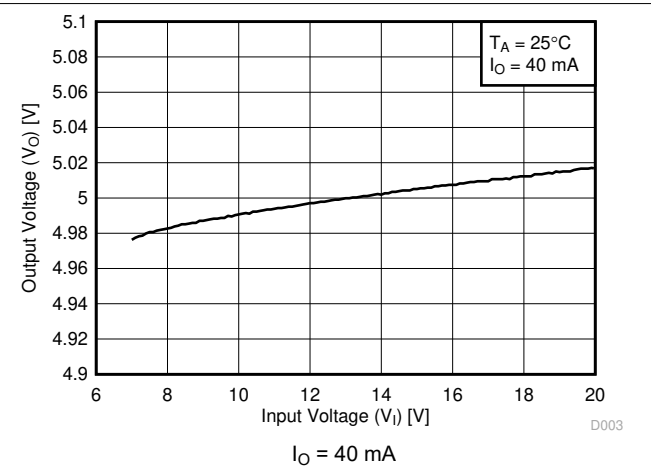
图 6-6. Line Regulation at I_O = 40\text{ mA} for Legacy Chip
