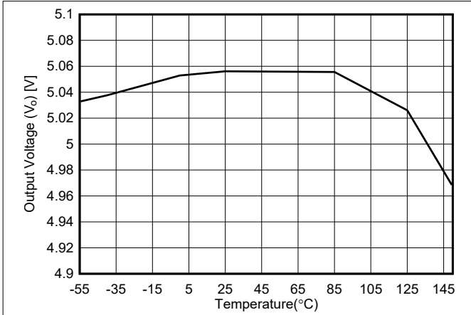
图 6-1. V_O vs Temperature for New Chip
