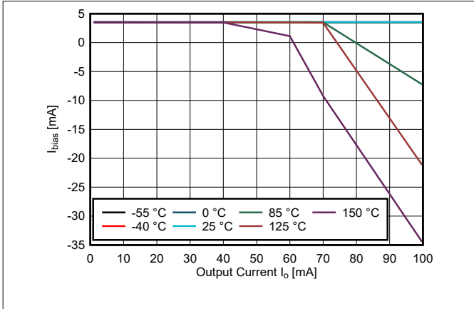
图 6-13. Bias Current vs Load Current for New Chip
