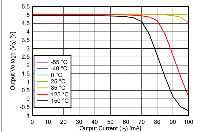
图 6-3. Load Regulation for Legacy Chip
