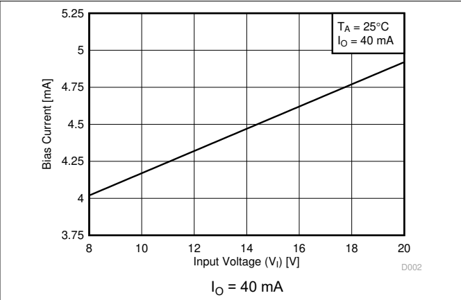
图 6-14. Bias Current vs Input Voltage for Legacy Chip
