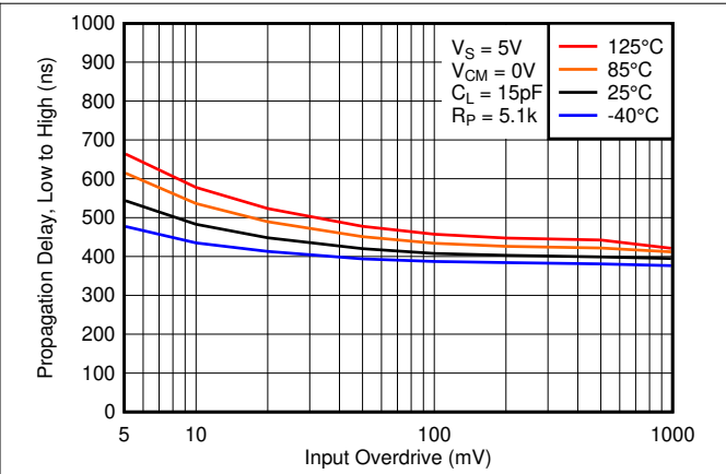
Figure 6-31. Low to High Propagation Delay vs. Input Overdrive Voltage, 5V
