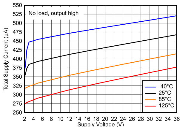
Figure 6-6. Total Supply Current vs. Supply Voltage
