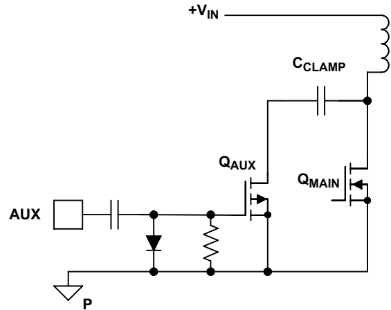
Figure 24. Low-Side P-Channel
