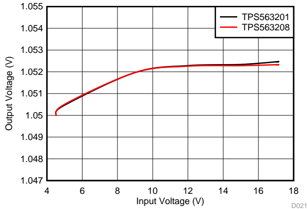
Figure 22. TPS563201 and TPS563208 Line Regulation
