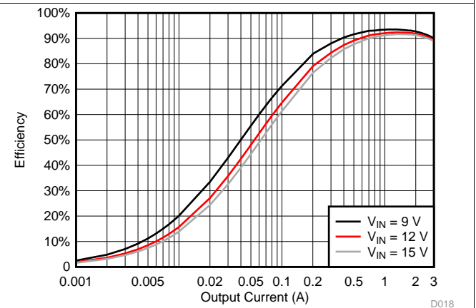
Figure 16. TPS563208 V_{OUT} = 1.8\text{ V} Efficiency, L = 2.2\ \mu\text{H}
