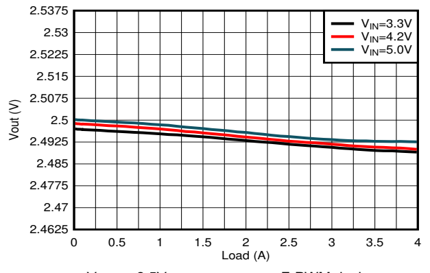
Figure 8-18. Load Regulation
