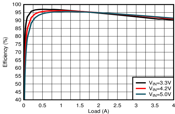
Figure 8-15. Efficiency
