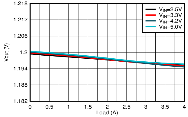
V_{OUT} = 1.2V F-PWM devices Figure 8-10. Load Regulation
