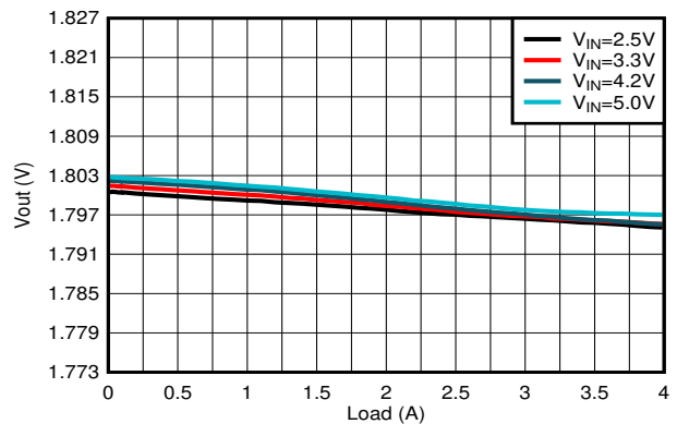
V_{OUT} = 1.8V F-PWM devices Figure 8-14. Load Regulation
