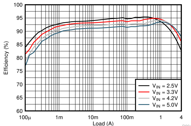
V_{OUT} = 1.8V D004 Figure 8-11. Efficiency
