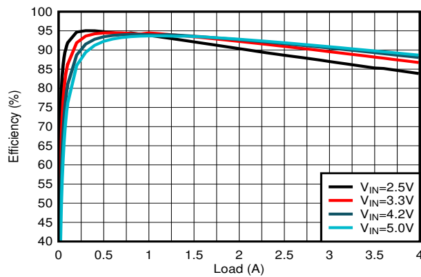
V_{OUT} = 1.8V F-PWM devices Figure 8-13. PWM Efficiency
