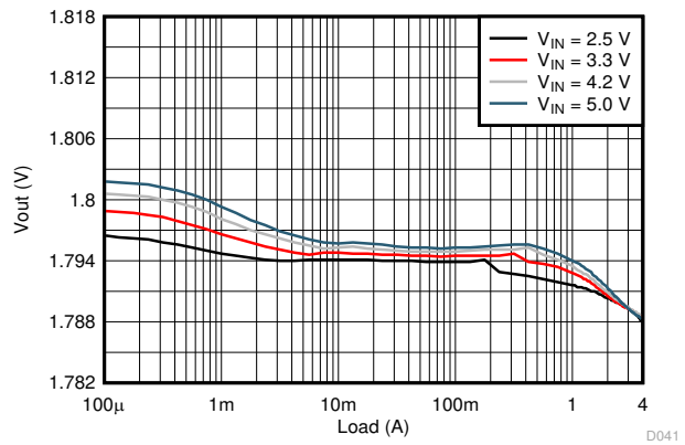
V_{OUT} = 1.8V D041 Figure 8-12. Load Regulation
