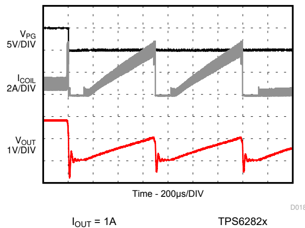
Figure 8-47. HICCUP Short-Circuit Protection
