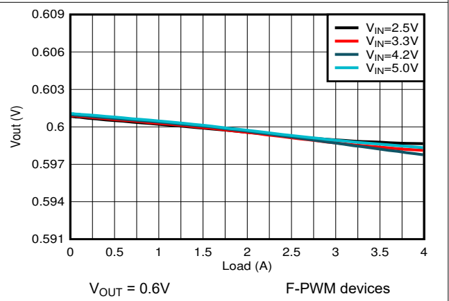
Figure 8-6. Load Regulation
