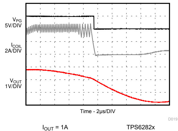
Figure 8-48. HICCUP Short-Circuit Protection (Zoom In)
