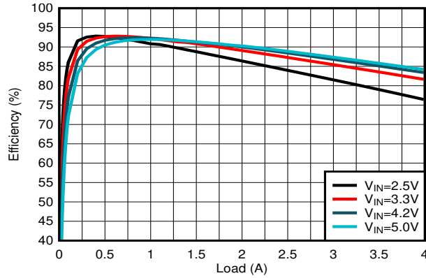
V_{OUT} = 1.2V F-PWM devices Figure 8-9. PWM Efficiency
