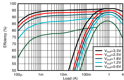
Efficiency at V_{IN} = 5V
