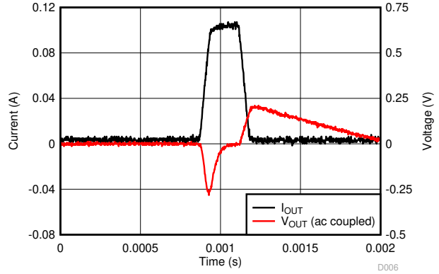
V_{OUT} = 5\text{ V} , C_{IN} = 1\ \mu\text{F} , C_{OUT} = 1\ \mu\text{F} , I_{OUT} = 1\text{ mA} \rightarrow 100\text{ mA} → 1\text{ mA} , Slew rate = 1\text{ mA}/\mu\text{s}
