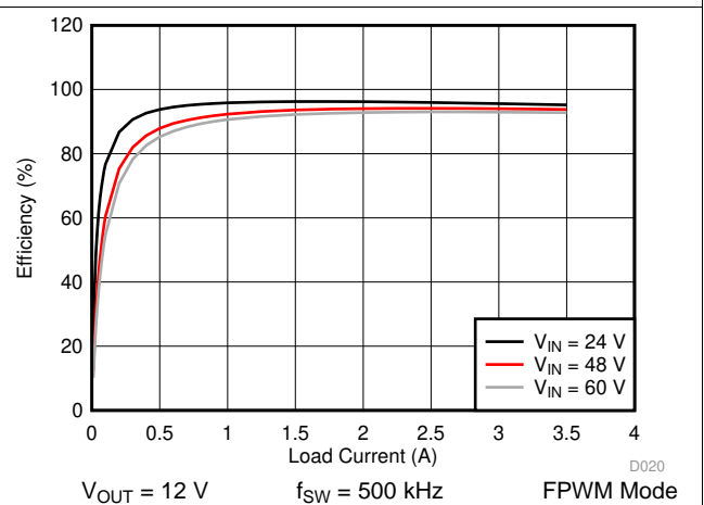
Figure 32. LM76003-Q1 Efficiency
