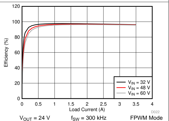
Figure 34. LM76003-Q1 Efficiency
