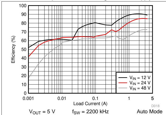
Figure 29. LM76003-Q1 Efficiency
