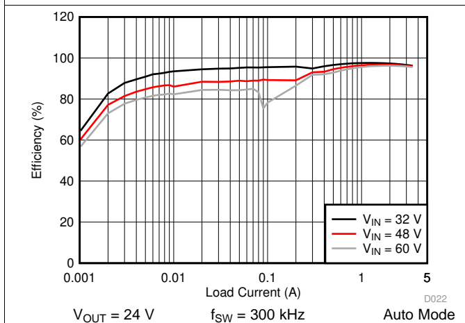
Figure 33. LM76003-Q1 Efficiency
