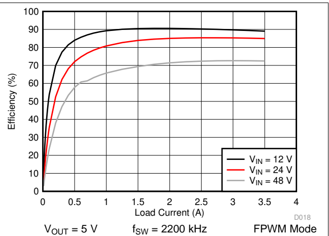
Figure 30. LM76003-Q1 Efficiency
