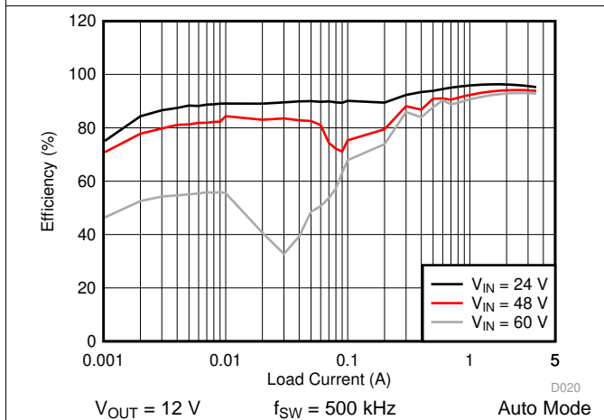
Figure 31. LM76003-Q1 Efficiency
