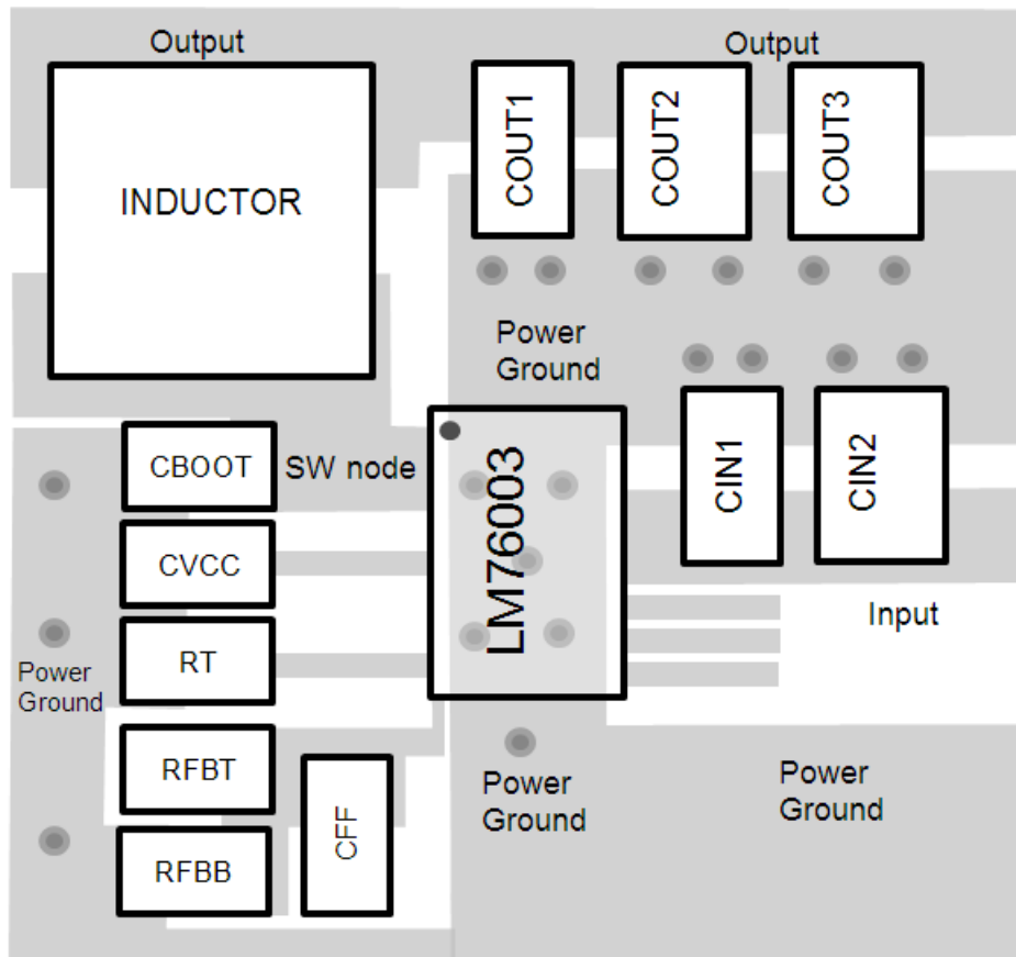
Figure 91. LM76002-Q1/LM76003-Q1 Layout
