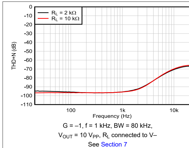
Figure 6-13. THD+N Ratio vs Frequency, G = -1
