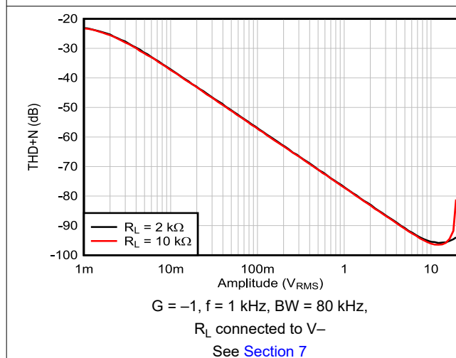
Figure 6-15. THD+N vs Output Amplitude, G = -1
