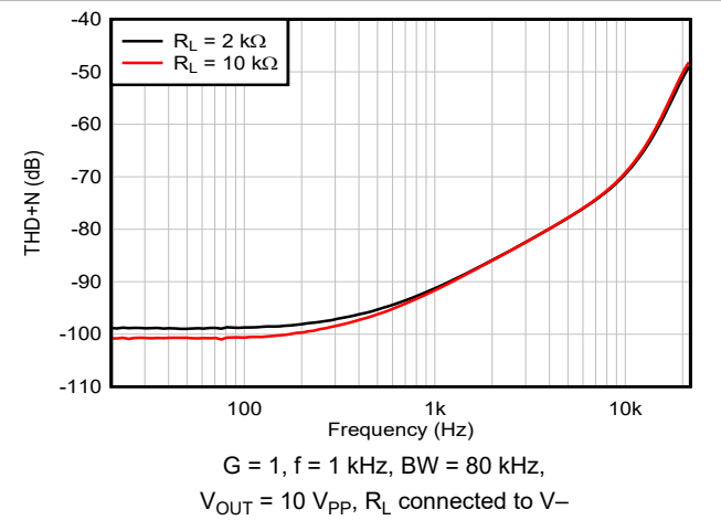
Figure 6-12. THD+N Ratio vs Frequency, G = 1
