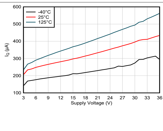
Figure 6-16. Quiescent Current vs Supply Voltage
