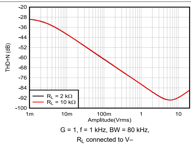
Figure 6-14. THD+N vs Output Amplitude, G = 1
