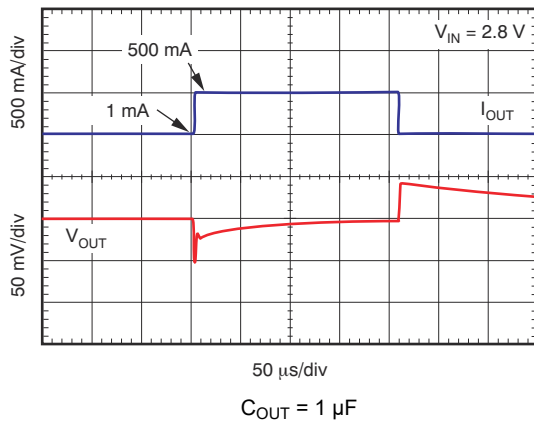
Figure 6-15. Load Transient Response 1 mA to 500 mA
