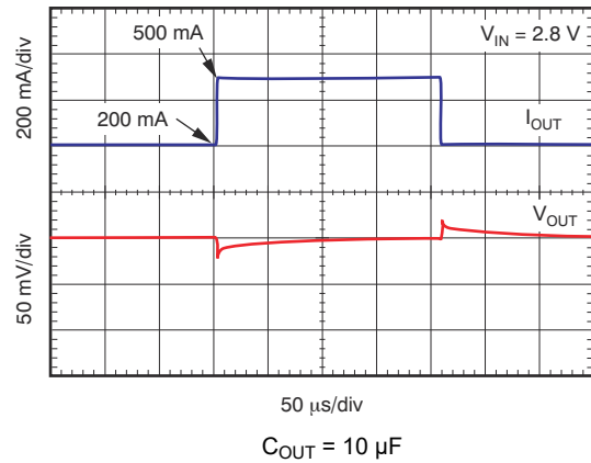
Figure 6-14. Load Transient Response 200 mA to 500 mA
