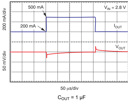
Figure 6-13. Load Transient Response 200 mA to 500 mA
