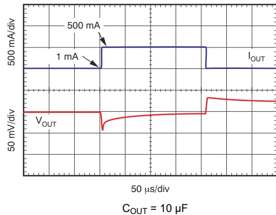
Figure 6-16. Load Transient Response 1 mA to 500 mA
