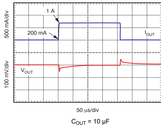
Figure 6-18. Load Transient Response 200 mA to 1 A
