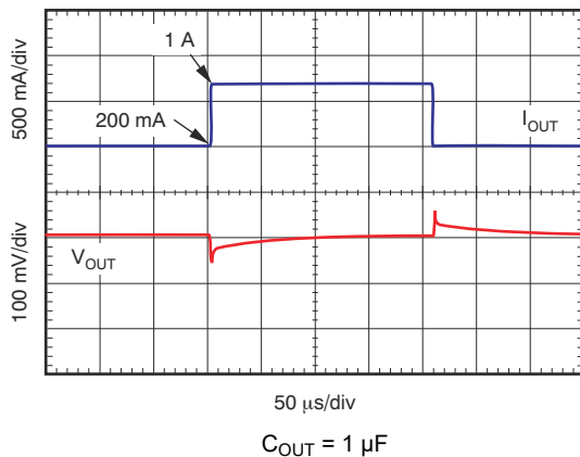
Figure 6-17. Load Transient Response 200 mA to 1 A
