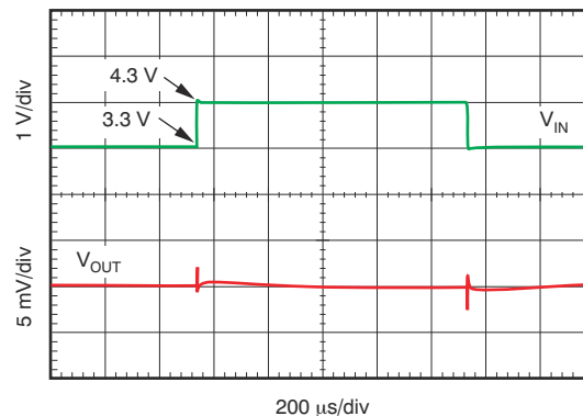
Figure 8-3. Line Transient Response V_{OUT} = 1.8\ \text{V} , I_{OUT} = 500\ \text{mA}
