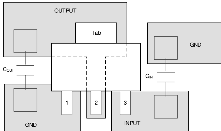
Figure 8-4. Layout Example
