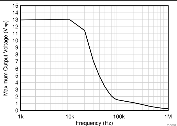
Figure 6-36. Maximum Output Voltage vs Frequency V_S = 15\text{ V}
