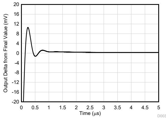
Figure 6-31. Large-Signal Step Response (Rising) G = 1, R_L = \text{open}
