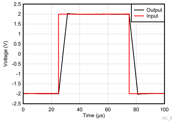
Figure 6-33. Large-Signal Step Response G = 1, R_L = \text{open}
