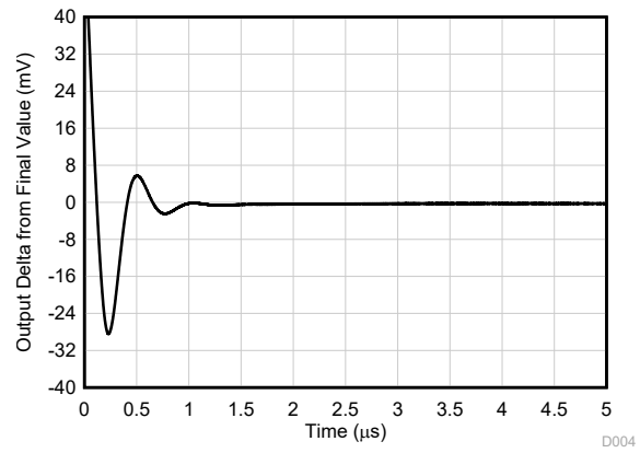
Figure 6-32. Large-Signal Step Response (Falling) G = 1, R_L = \text{open}
