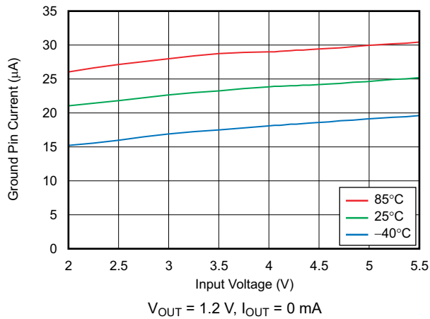
Figure 6-17. Ground Pin Current vs Input Voltage
