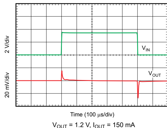
Figure 8-7. Line Transient Response
