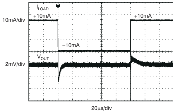
C_L = 1 \mu\text{F} , I_{\text{OUT}} = 10 \text{mA} Figure 7-17. Load Transient
