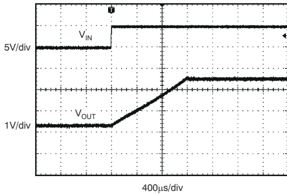
REF5025, C_L = 10 \mu\text{F} Figure 7-15. Start-Up
