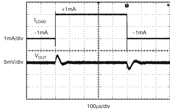
C_L = 10 \mu\text{F} , I_{\text{OUT}} = 1 \text{mA} Figure 7-18. Load Transient
