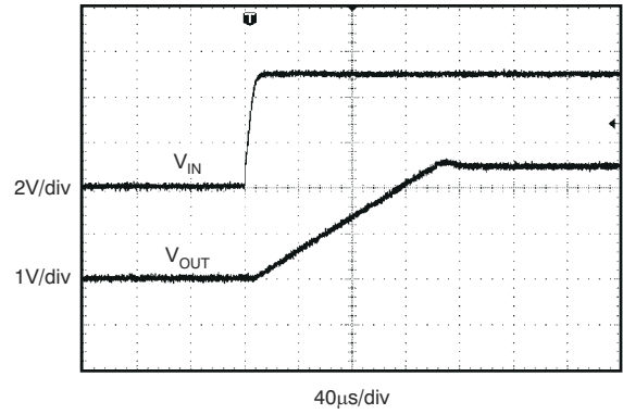
REF5025, C_L = 1 \mu\text{F} Figure 7-14. Start-Up
