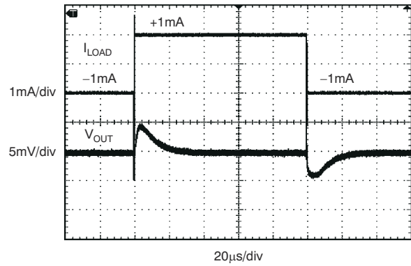
C_L = 1 \mu\text{F} , I_{\text{OUT}} = 1 \text{mA} Figure 7-16. Load Transient
