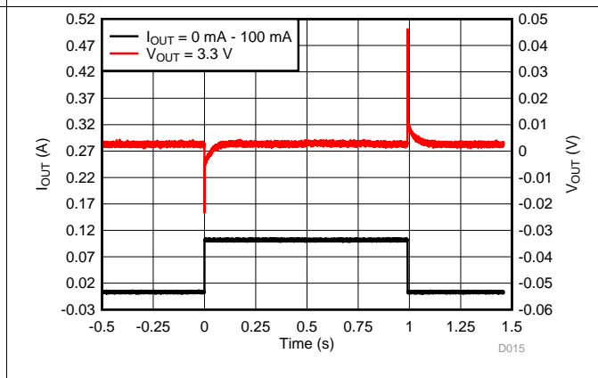
Figure 16. Load Transient
