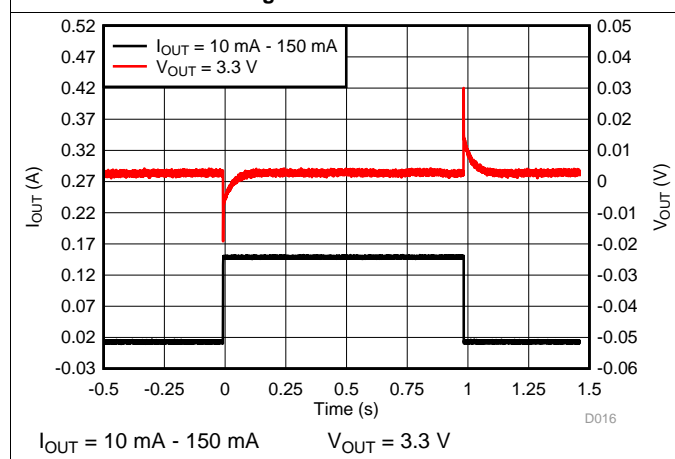
Figure 17. Load Transient
