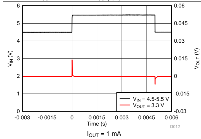
Figure 13. Line Transient
