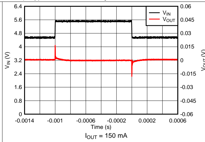
Figure 14. Line Transient
