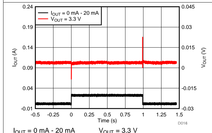
Figure 15. Load Transient
