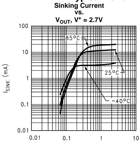
V_{OUT} from V^- (V) Figure 10.
