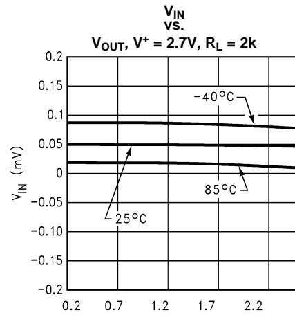
V_{OUT} (V) Figure 13.
