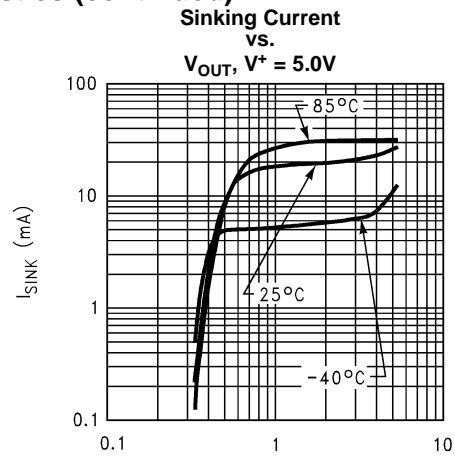
V_{OUT} from V^- (V) Figure 11.
