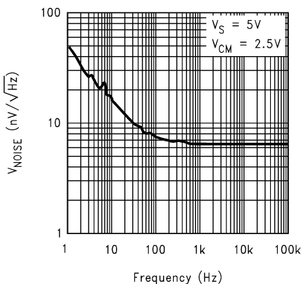
Figure 2. Voltage Noise
