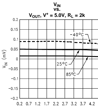
V_{OUT} (V) Figure 14.
