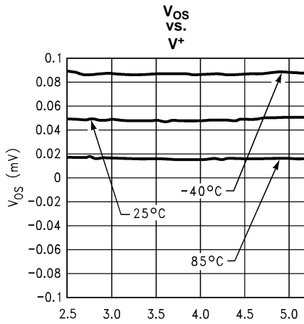
Supply Voltage (V) Figure 12.
