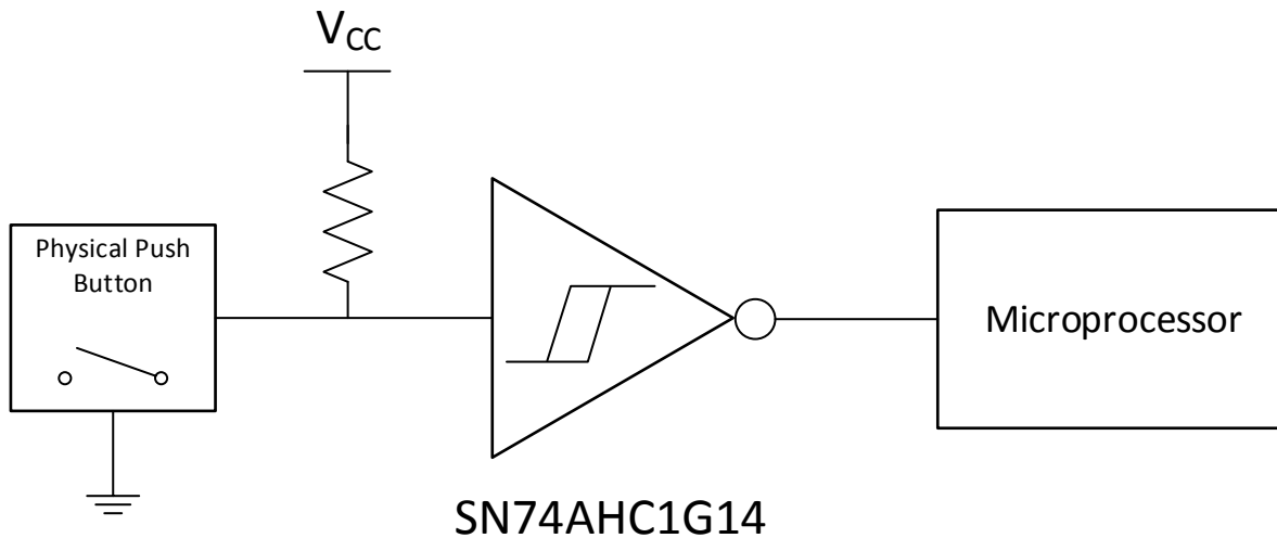
Figure 8-1. Switch Debouncer
