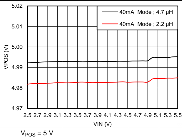
Figure 47. Line Regulation
