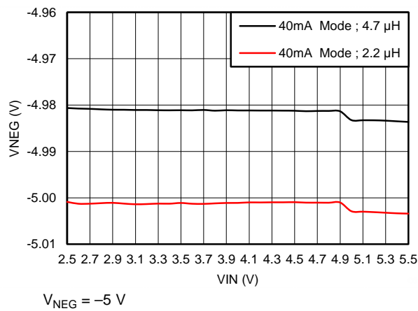
Figure 49. Line Regulation
