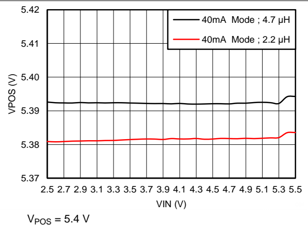
Figure 48. Line Regulation
