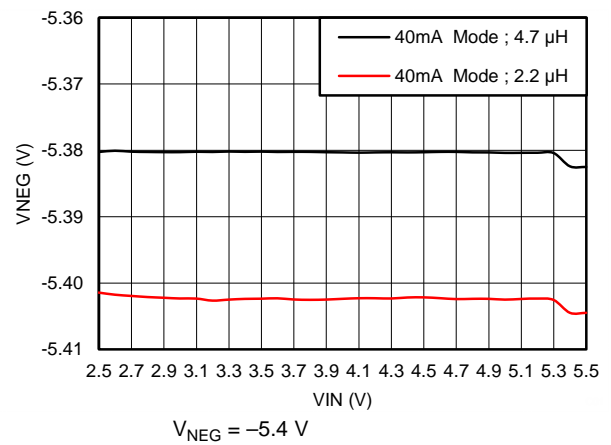
Figure 50. Line Regulation
