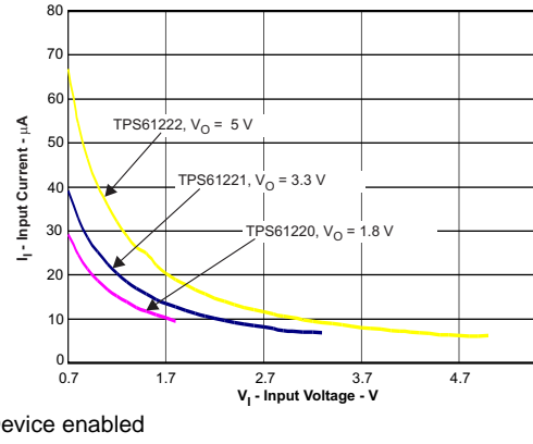
Figure 8. No Load Input Current versus Input Voltage, Device Enabled (TPS61220, TPS61221, TPS61222)
