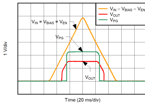
图 6-45. Power-Up and Power-Down
