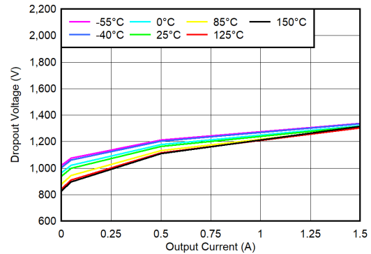
图 6-31. V BIAS Dropout Voltage vs I OUT and Temperature (T J )
