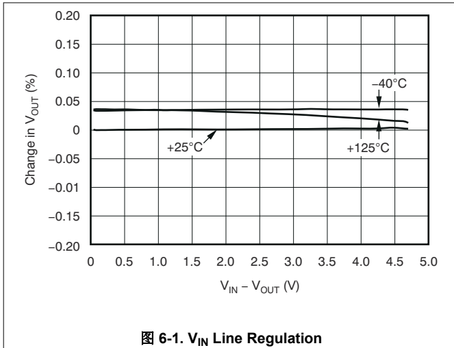
图 6-1. V_{IN} Line Regulation
