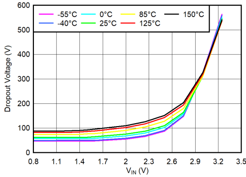
图 6-28. V IN Dropout Voltage vs V IN and Temperature (T J ) for I OUT = 1.5 A
