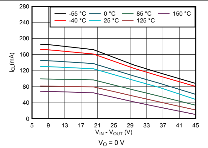
图 6-18. I_{SC} vs V_I for New Chip
