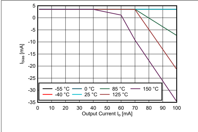
图 6-13. Bias Current vs Load Current for New Chip
