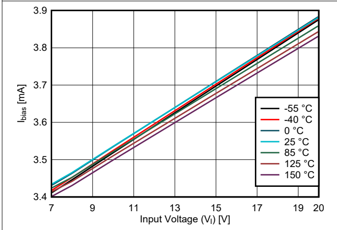
图 6-17. Bias Current vs Input Voltage at I_O = 1\text{ mA} for New Chip
