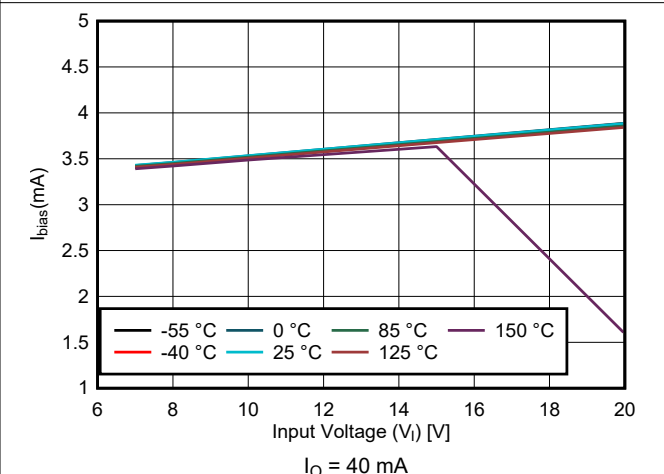
图 6-16. Bias Current vs Input Voltage for New Chip
