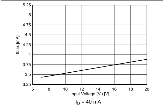
图 6-15. Bias Current vs Input Voltage for New Chip at T_J = 25^\circ\text{C}
