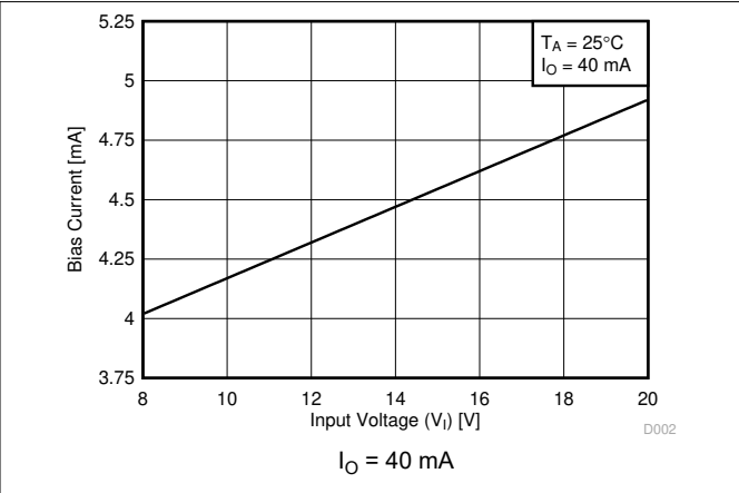
图 6-14. Bias Current vs Input Voltage for Legacy Chip
