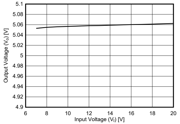
图 6-8. Line Regulation at I_O = 1\text{ mA} for New Chip at T_J = 25\text{ }^\circ\text{C}
