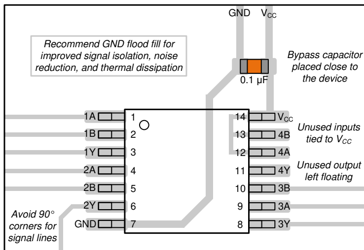
Figure 9-3. Example Layout for the SN74AHC1G04-Q1
