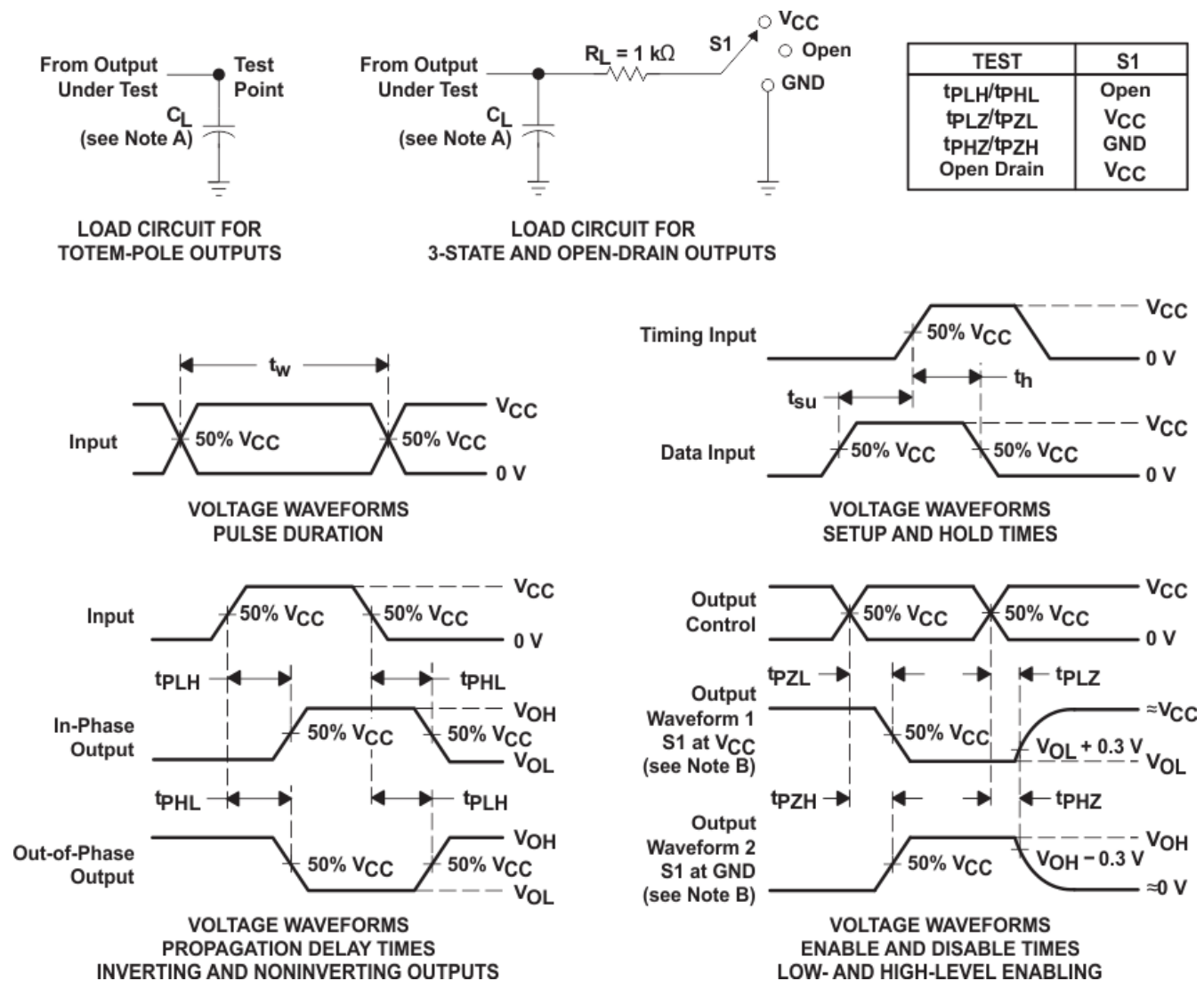
Figure 7-1. Load Circuit And Voltage Waveforms
