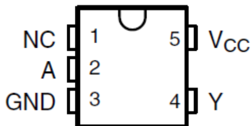
Figure 5-1. DBV or DCK Package (Top View)
