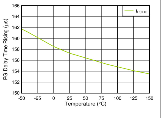
图 6-18. t_{PGDH} vs Temperature
