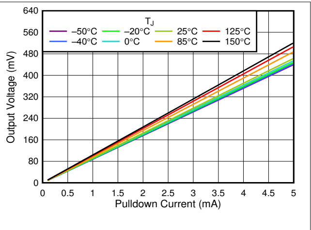
图 6-14. V_{OUT} vs I_{OUT} Pulldown Resistor
