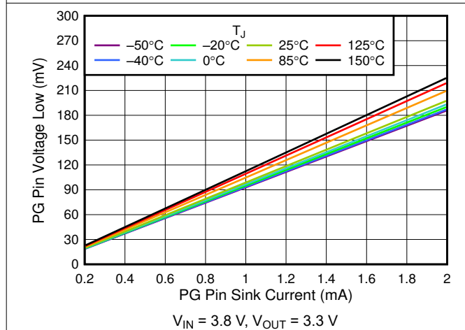
图 6-17. V_{OL(PG)} vs PG Pin Sink Current
