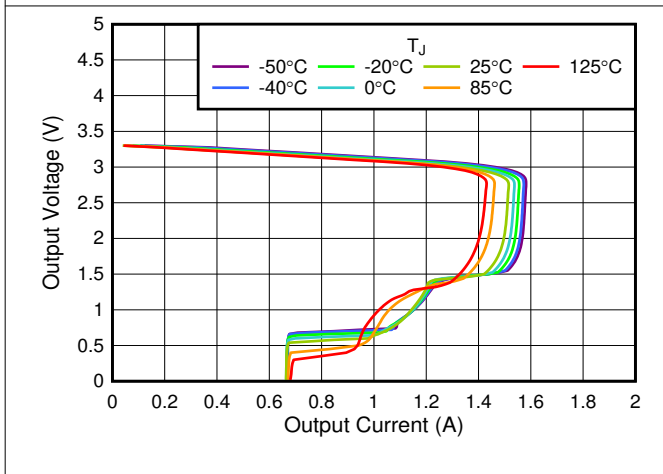
图 6-23. 3.3-V Foldback Current Limit vs I_{OUT}
