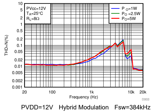
图 8-3. THD+N vs Frequency
