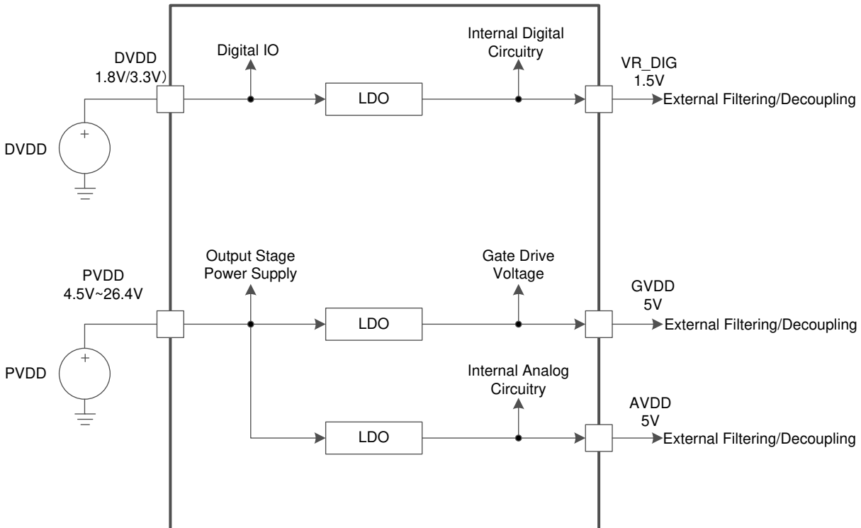
图 9-1. Power Supply Function Block Diagram
