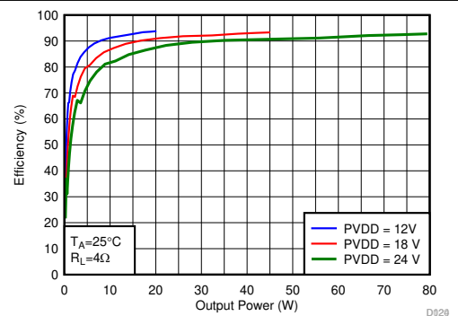
A. Hybrid Modulation F SW = 384 kHz Load = 4 Ω PBTL Mode
