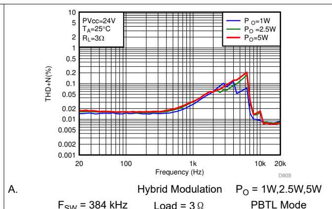
图 6-28. THD+N vs Frequency-PBTL
