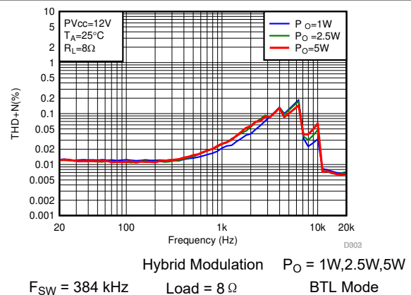
图 6-4. THD+N vs Frequency-BTL
