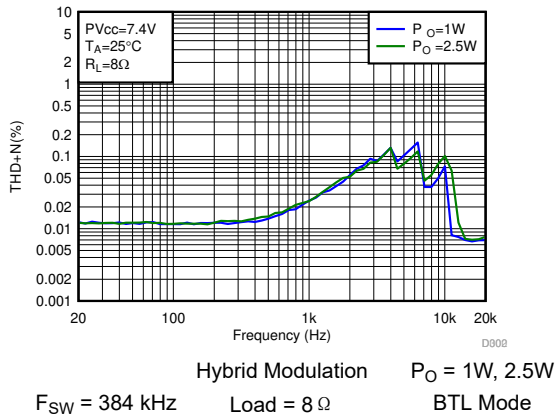
图 6-1. THD+N vs Frequency-BTL
