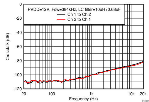
A. PVDD=12V Hybrid Modulation F_{SW} = 384 \text{ kHz} Load = 6 \Omega BTL Mode
