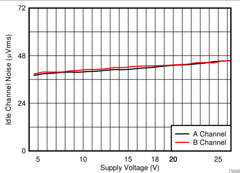
A. BD Modulation F SW = 768 kHz Load = 6 Ω BTL Mode
