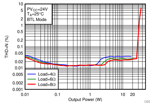
A. BD Modulation 2 Channel Run F_{SW} = 768 \text{ kHz} Load = 4 \Omega, 6 \Omega, 8 \Omega BTL Mode
