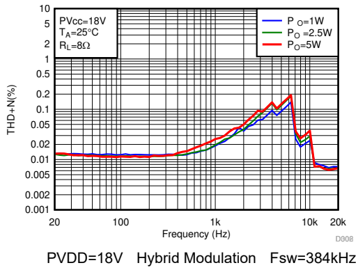
图 8-4. THD+N vs Frequency
