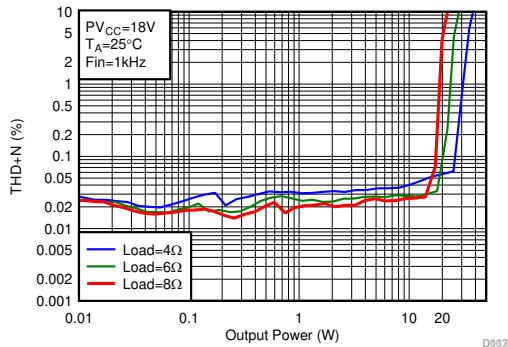
A. One channel run Hybrid Modulation F_{in} = 1 \text{ kHz} F_{SW} = 384 \text{ kHz} Load = BTL Mode 4 \Omega / 6 \Omega / 8 \Omega
