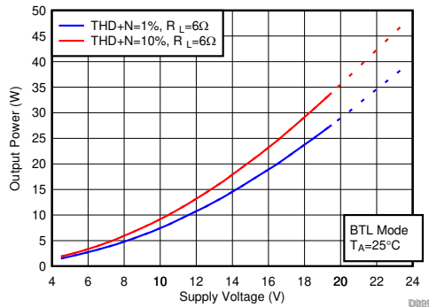
A. Dashed lines represent thermally limited region. BD Modulation F SW = 768 kHz Load = 6 Ω BTL Mode
