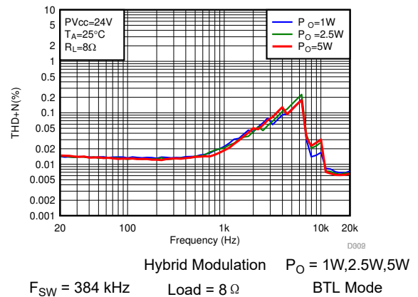
图 6-10. THD+N vs Frequency-BTL
