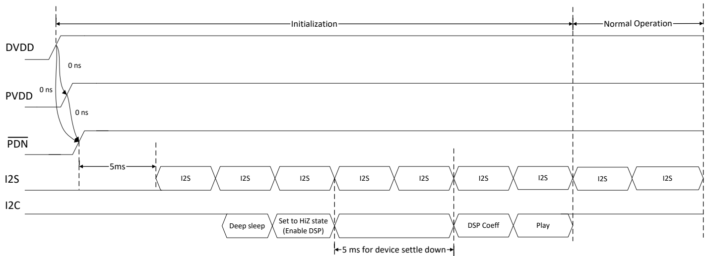
图 7-14. Start-up Sequence
