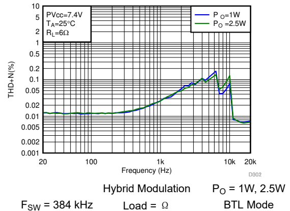
图 6-2. THD+N vs Frequency-BTL
