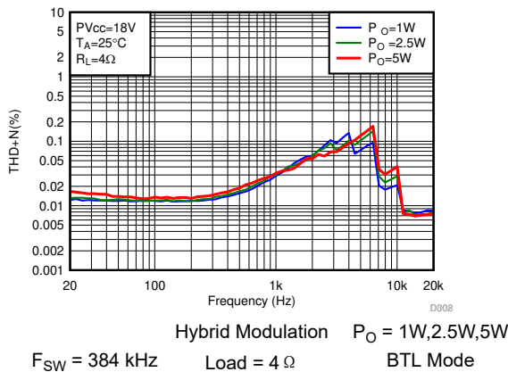
图 6-9. THD+N vs Frequency-BTL
