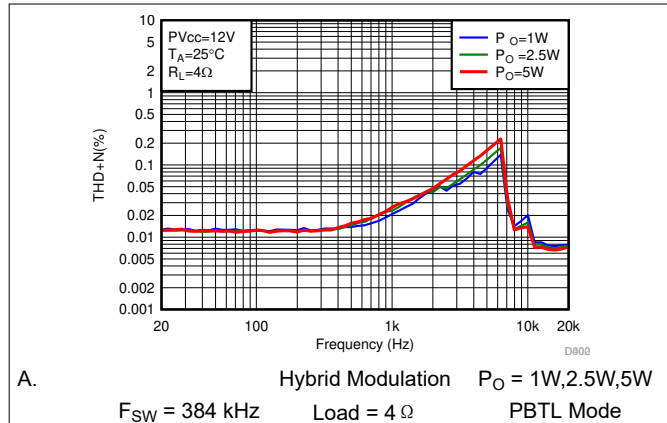
图 6-23. THD+N vs Frequency-PBTL
