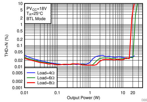
A. BD Modulation Two Channel Run F_{SW} = 768 \text{ kHz} Load = 4 \Omega, 6 \Omega, 8 \Omega BTL Mode
