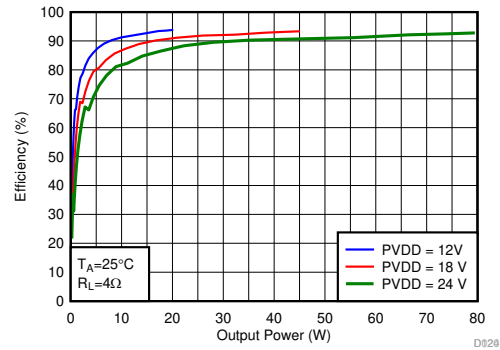
图 8-11. Efficiency vs Output Power
