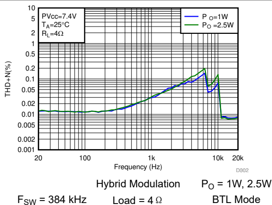
图 6-3. THD+N vs Frequency-BTL
