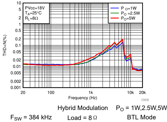
图 6-7. THD+N vs Frequency-BTL
