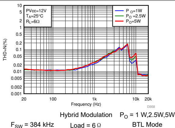
图 6-5. THD+N vs Frequency-BTL
