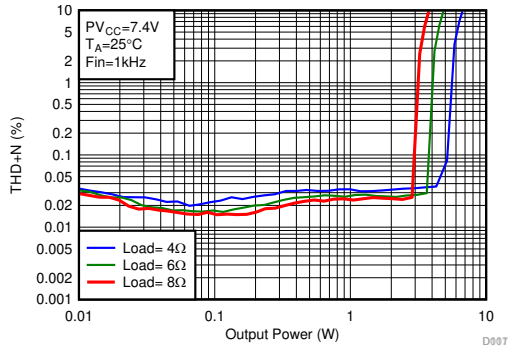
A. Hybrid Modulation F_{in} = 1 \text{ kHz} F_{SW} = 384 \text{ kHz} Load = BTL Mode 4 \Omega / 6 \Omega / 8 \Omega
