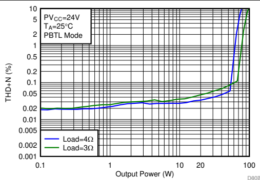
A. Hybrid Modulation F SW = 384 kHz Load = 4 Ω, 3 Ω PBTL Mode
