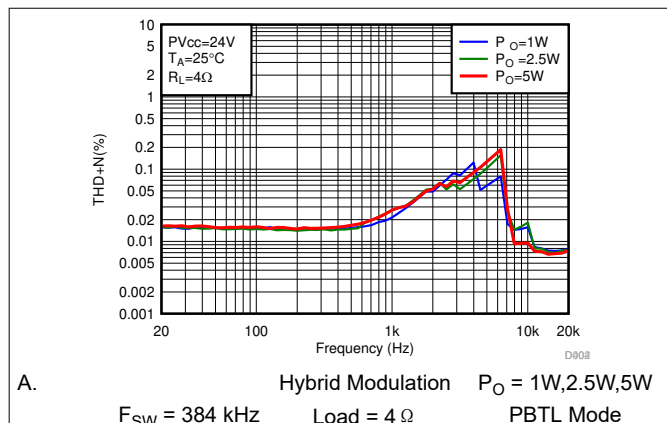
图 6-27. THD+N vs Frequency-PBTL
