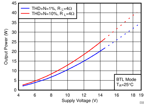
A. Dashed lines represent thermally limited region. BD Modulation F SW = 768 kHz Load = 4 Ω BTL Mode
