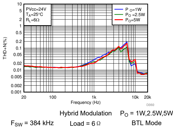
图 6-11. THD+N vs Frequency-BTL
