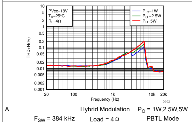
图 6-25. THD+N vs Frequency-PBTL
