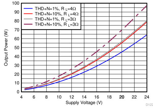
图 6-35. Output Power vs Supply Voltage
