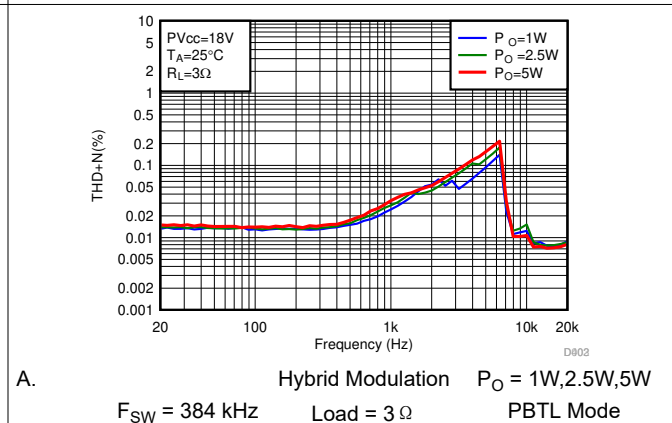
图 6-26. THD+N vs Frequency-PBTL
