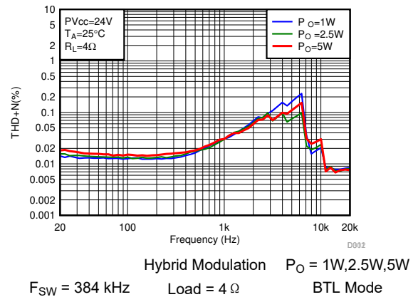
图 6-12. THD+N vs Frequency-BTL
