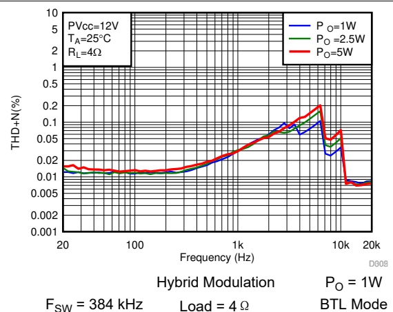
图 6-6. THD+N vs Frequency-BTL
