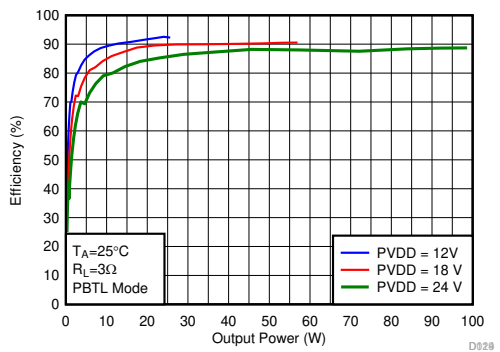
A. Hybrid Modulation F SW = 384 kHz Load = 3 Ω PBTL Mode
