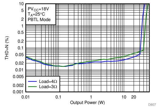
A. Hybrid Modulation F SW = 384 kHz Load = 4 Ω, 3 Ω PBTL Mode
