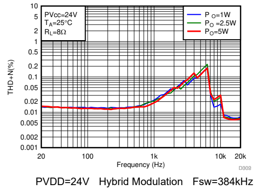
图 8-5. THD+N vs Frequency
