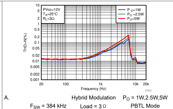
图 6-24. THD+N vs Frequency-PBTL
