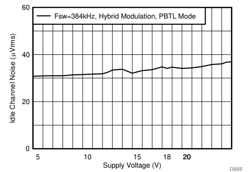
A. Hybrid Modulation F SW = 384 kHz Load = 6 Ω PBTL Mode
