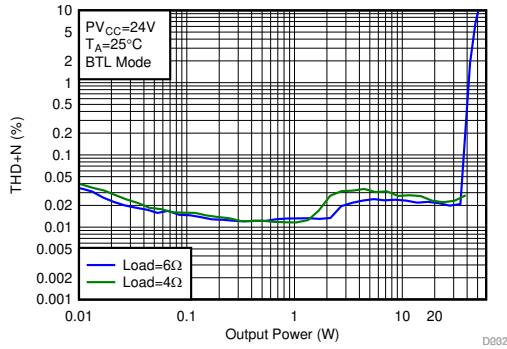
A. BD Modulation 1 Channel Run F SW = 768 kHz Load = 4 Ω, 6 Ω BTL Mode
