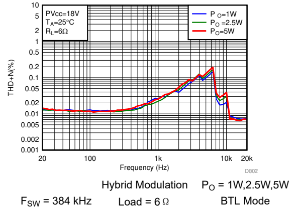
图 6-8. THD+N vs Frequency-BTL
