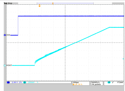
Figure 9-53. Start-Up Timing
