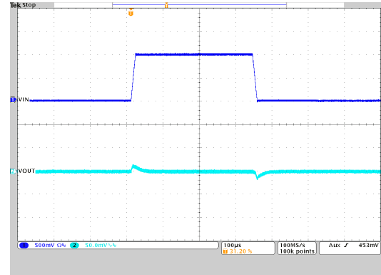
V_{OUT} = 1.0\text{ V} PWM T_A = 25^\circ\text{C} I_{OUT} = 2\text{ A} V_{IN} = 4.5\text{ V to } 5.5\text{ V to } 4.5\text{ V}
