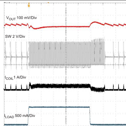
Time Base - 10 us/Div V_{IN} = 3.6\text{ V} V_{OUT} = 1.8\text{ V} I_{OUT} = 20\text{ to }750\text{ mA}
