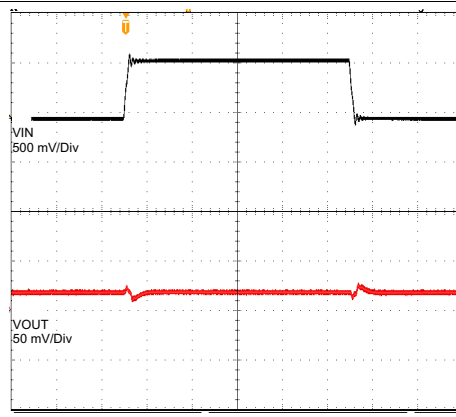
Time Base - 100 us/Div V_{IN} = 3.6\text{ to }4.2\text{ V} V_{OUT} = 1.8\text{ V} I_{OUT} = 500\text{ mA} C_{OUT} = 10\text{ }\mu\text{F} L = 1.2\text{ }\mu\text{H}
