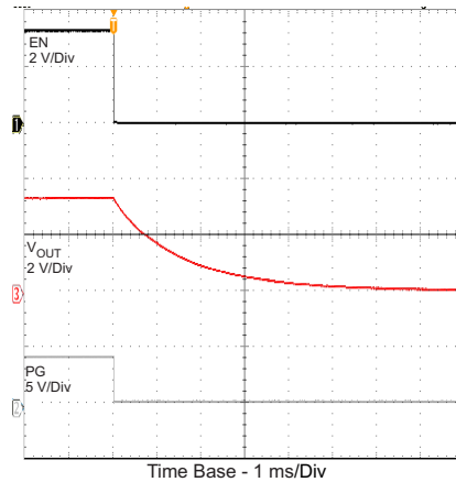
Time Base - 1 ms/Div V_{IN} = 4.2 V V_{OUT} = 3.3 V No load PG pullup resistor, 10 k \Omega
