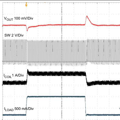
Time Base - 10 us/Div V_{IN} = 3.6\text{ V} V_{OUT} = 1.2\text{ V} I_{OUT} = 0.2\text{ to }1\text{ A}
