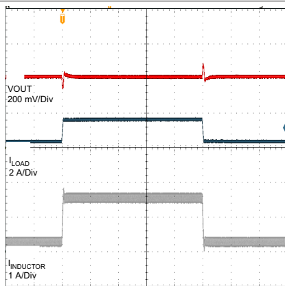
Time Base - 100 us/Div V_{IN} = 3.6\text{ V} V_{OUT} = 1.8\text{ V} L = 1.2\text{ }\mu\text{H} C_{OUT} = 10\text{ }\mu\text{F}
