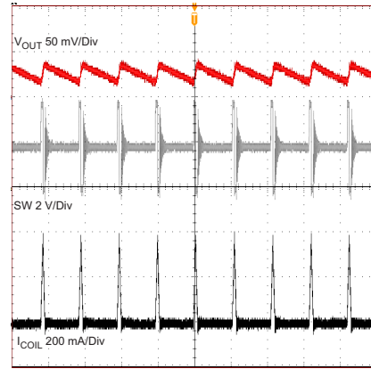
Time Base - 4 us/Div V_{IN} = 3.6\text{ V} V_{OUT} = 1.8\text{ V} MODE = GND C_{OUT} = 10\text{ }\mu\text{F} L = 1.2\text{ }\mu\text{H} I_{OUT} = 20\text{ mA}
