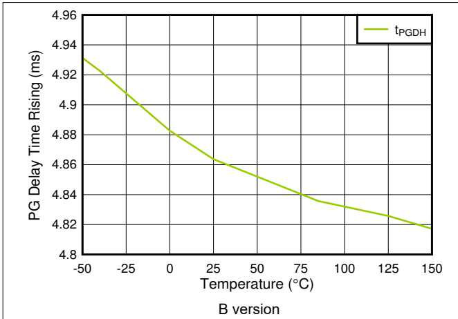
图 6-25. t_{PGDH} vs Temperature (For TPS746B Only)
