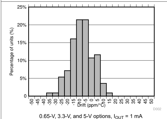
图 6-5. Temperature Drift Histogram (25°C to 150°C)
