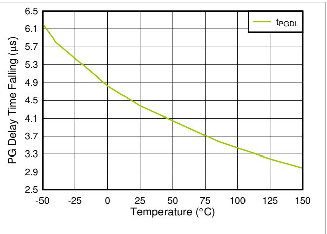
图 6-26. t_{PGDL} vs Temperature
