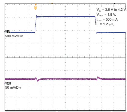
Time Base - 100 μs/Div Figure 20. Line Transient Response PWM Mode
