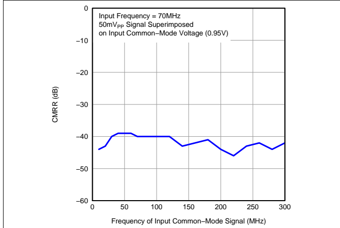
Figure 83. CMRR vs Frequency
