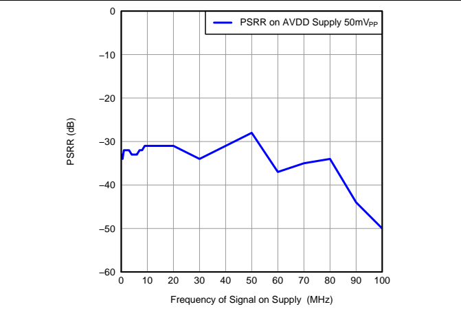
Figure 84. PSRR vs Frequency
