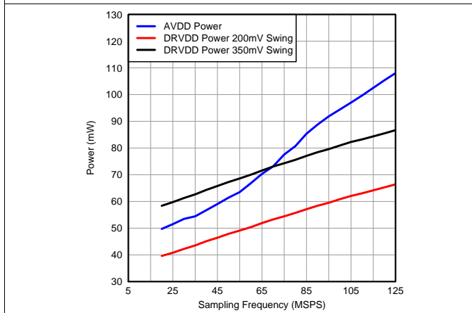
Figure 85. Power vs Sample Rate
