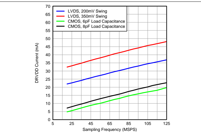
Figure 86. DRVDD Current vs Sample Rate
