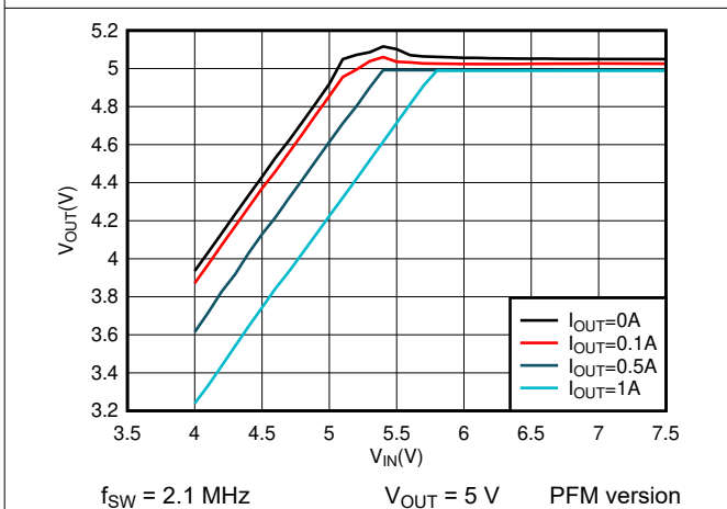
Figure 7-5. 5-V Dropout
