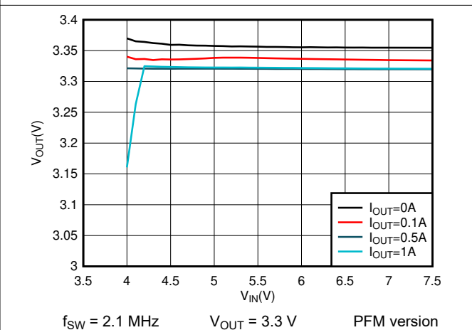
Figure 7-6. 3.3-V Dropout
