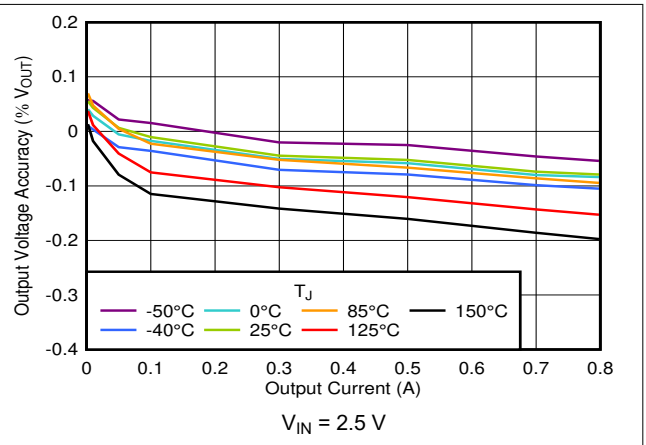
图 7-2. V_{OUT} Accuracy vs I_{OUT}
