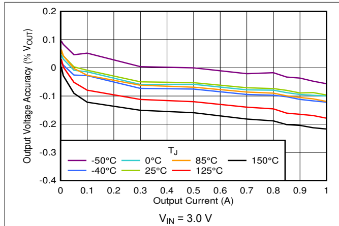
图 7-1. V_{OUT} Accuracy vs I_{OUT}
