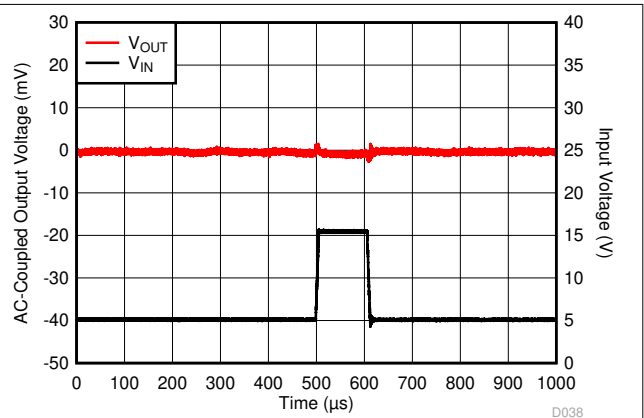
图 7-14. V_{IN} Transient From 5 V to 16 V
