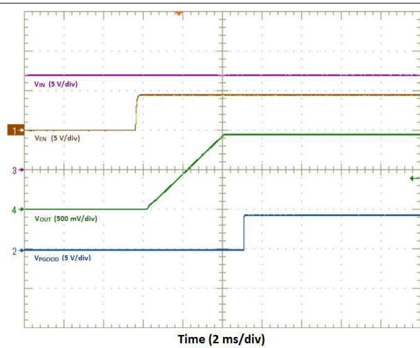
Figure 8-3. Start-Up Waveforms
