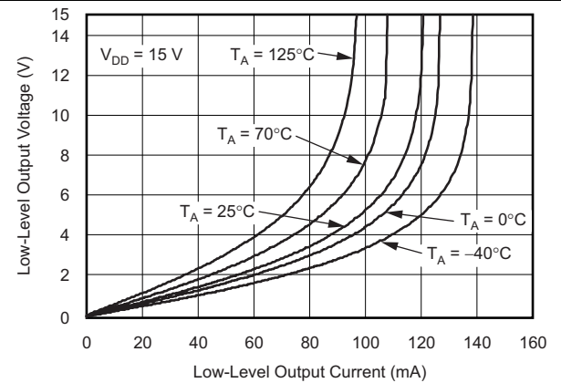
Figure 11. Low-Level Output Voltage vs Low-Level Output Current
