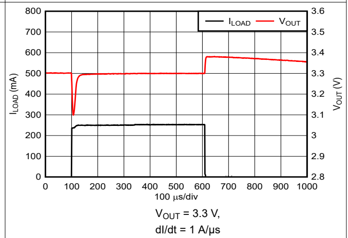
Figure 5-42. Load Transient Response for New Chip
