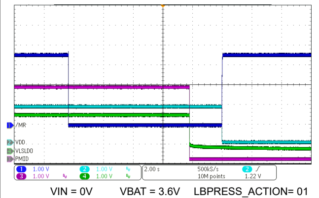
Figure 8-7. Ship Mode Entry with \overline{MR} Long Button Press
