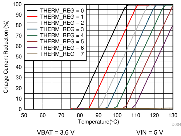
Figure 6-15. Charge Current Thermal Regulation
