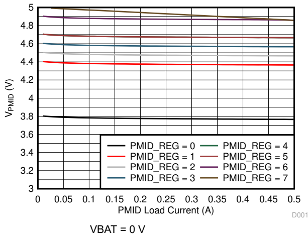
Figure 6-13. PMID Load Regulation
