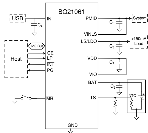
Simplified Schematic
