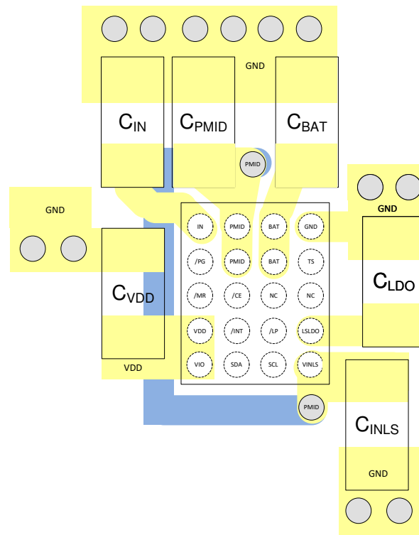
Figure 10-1. Layout Example
