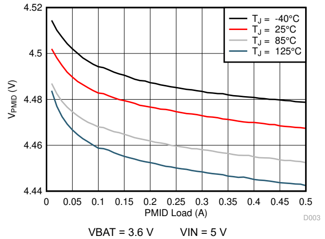
Figure 6-14. PMID Load Regulation vs. Temperature
