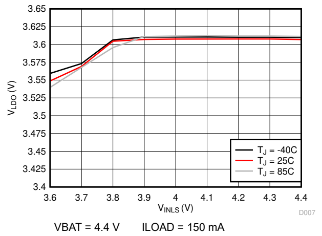
Figure 6-12. LDO Line Regulation (VLDO = 3.6 V)
