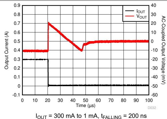
Figure 6-54. Load Transient
