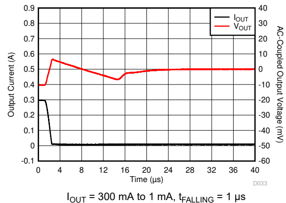
Figure 6-52. Load Transient
