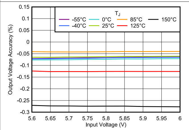
Figure 6-24. Output Voltage Accuracy vs V_{IN}
