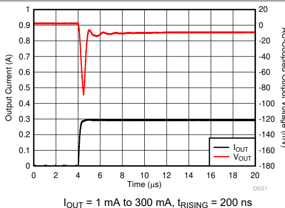
Figure 6-53. Load Transient
