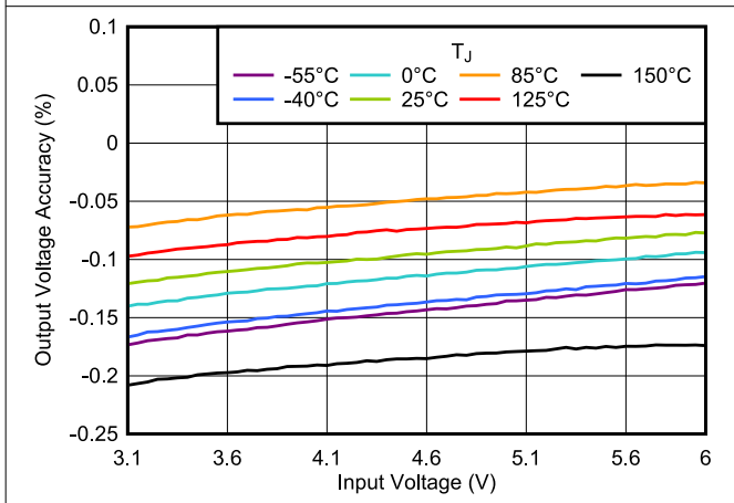
Figure 6-23. Output Voltage Accuracy vs V_{IN}
