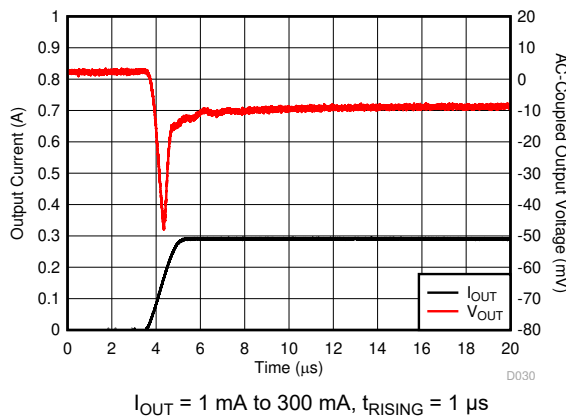
Figure 6-51. Load Transient
