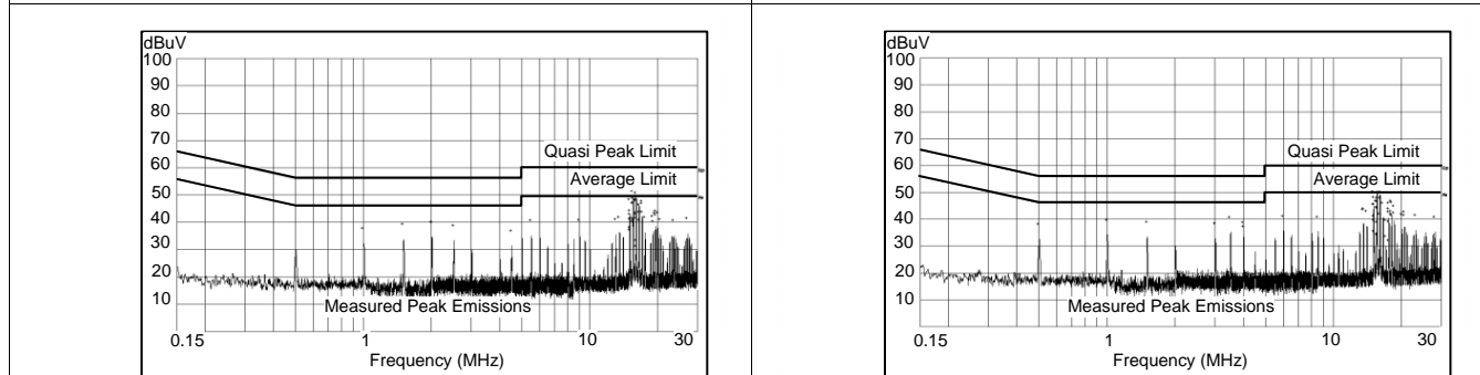
Figure 23. Conducted EMI Curve V_{OUT} = 3.3\text{ V} F_S = 500\text{ kHz} I_{OUT} = 0.5\text{ A} Measured on the LM46000PWPEVM with default BOM. EVM input filter: L_{in} = 1\text{ }\mu\text{H} C_d = 47\text{ }\mu\text{F} C_{IN4} = 68\text{ }\mu\text{F}
