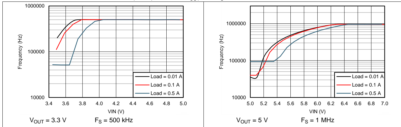
Figure 19. Switching Frequency vs V_{IN} in Dropout Operation
