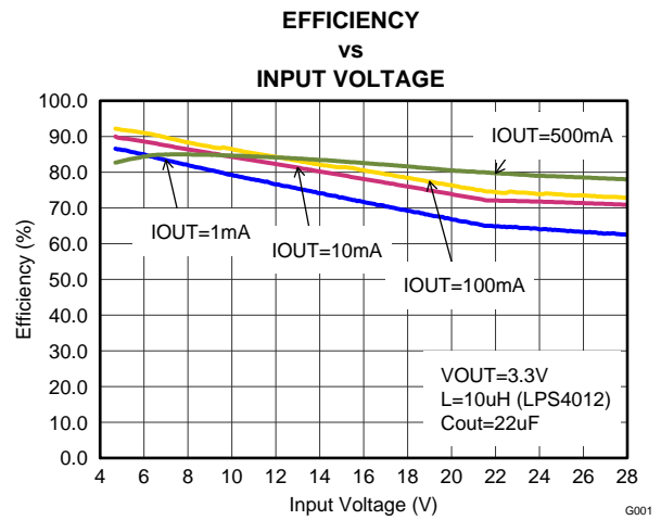
Figure 10. Vout=3.3V
