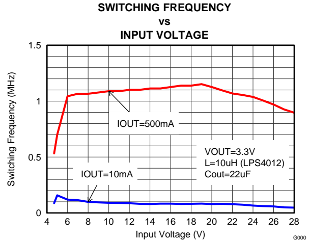
Figure 24. Switching Frequency
