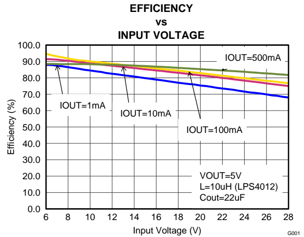
Figure 6. Vout=5V
