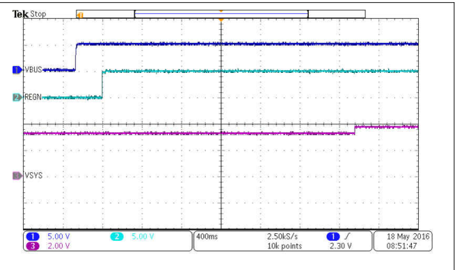
Figure 9-3. Power Up with Charge Disabled
