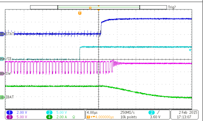
Figure 9-7. Charge Disable
