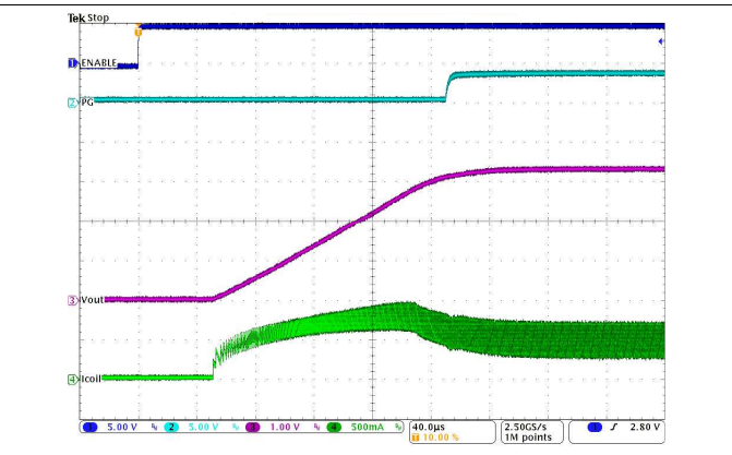
Figure 31. Startup with I_{OUT} = 500\text{ mA} , V_{OUT} = 3.3\text{ V}
