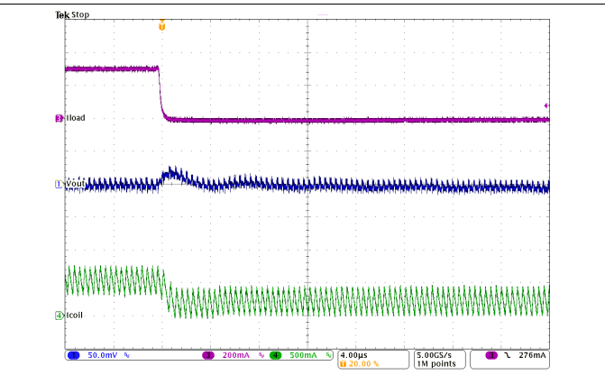
Figure 29. Load Transient Response in PWM Mode (200 mA to 500 mA), Falling Edge
