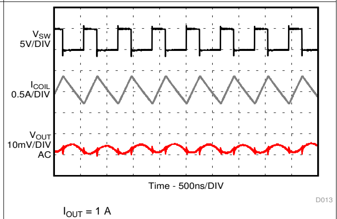
Figure 20. PWM Operation
