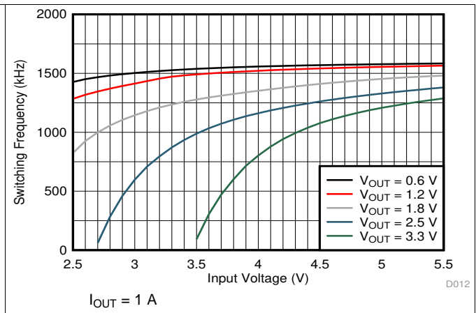
Figure 18. Switching Frequency vs Input Voltage
