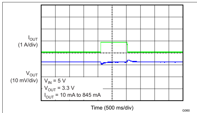
Figure 19. Load Transient
