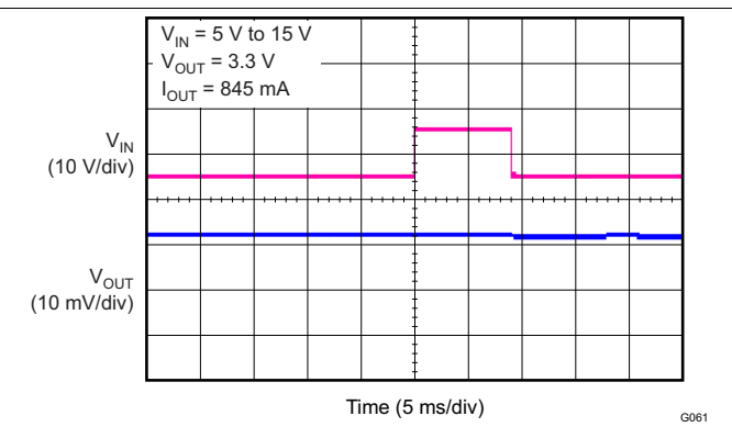
Figure 20. Line Transient
