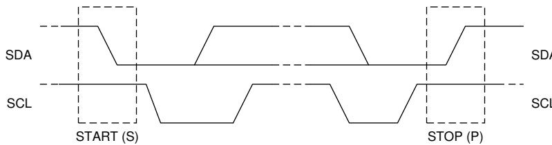
Figure 8-8. TS START and STOP conditions
