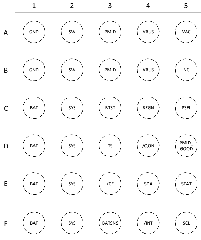
Figure 6-1. BQ25618 YFF Package 30-Pin WCSP Top View
