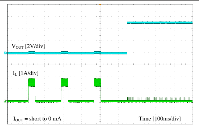
Figure 9-10. Short Recovery
