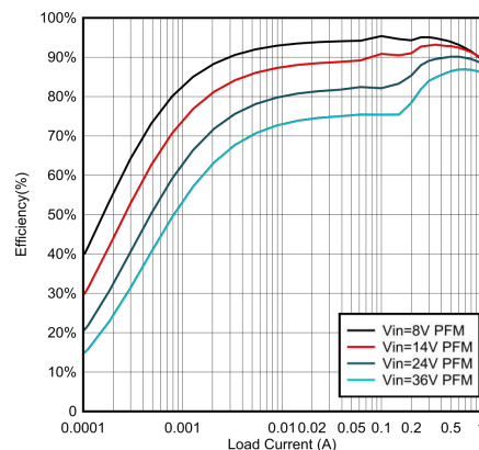
Efficiency Versus Output Current; V_{OUT} = 5\text{ V}, 1100\text{ kHz}
