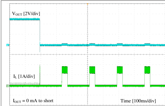
Figure 9-9. Short Protection
