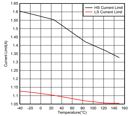
Figure 7-14. HS and LS Current Limit Versus Temperature
