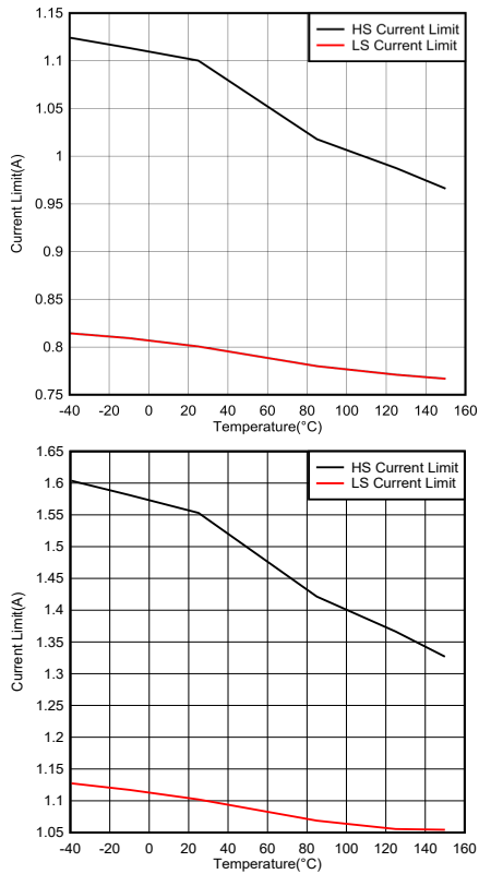
Figure 7-13. HS and LS Current Limit Versus Temperature
