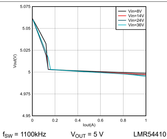
Figure 7-7. 5-V Load Regulation
