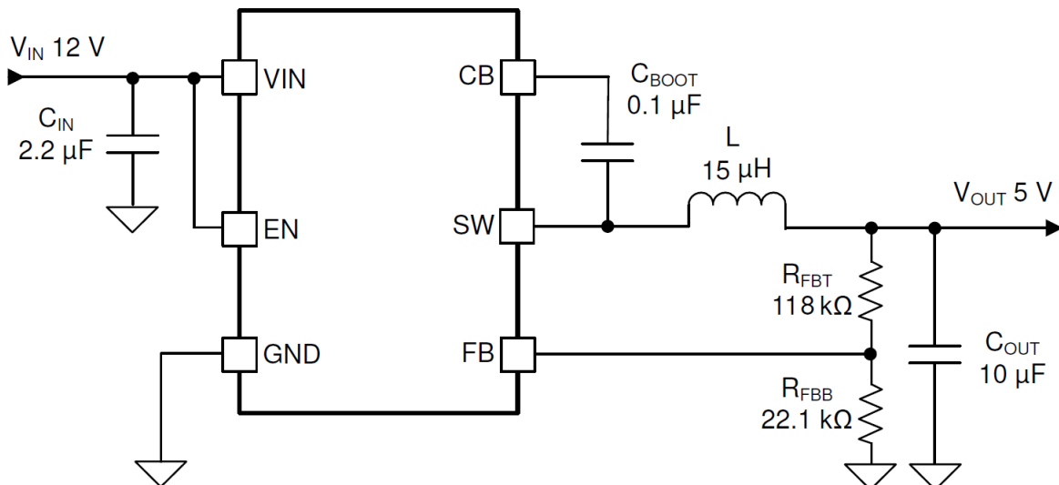
Figure 9-1. Application Circuit
