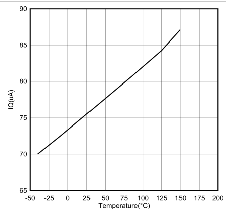
Figure 7-10. I_Q Versus Temperature
