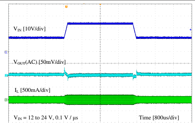
Figure 9-8. Line Transient
