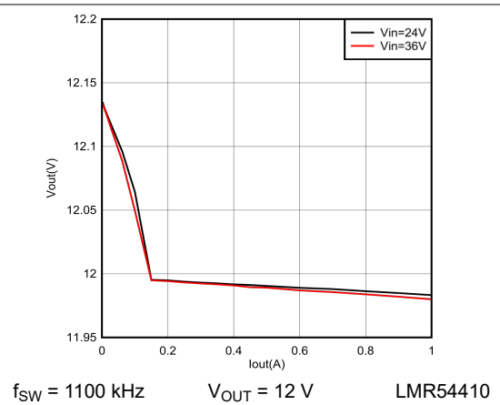
Figure 7-8. 12-V Load Regulation
