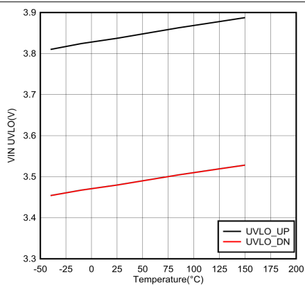
Figure 7-11. V_{IN} UVLO Versus Temperature
