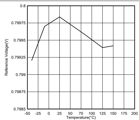
Figure 7-12. Reference Voltage Versus Temperature
