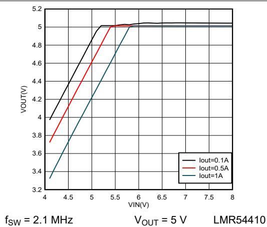
Figure 7-9. 5-V Dropout
