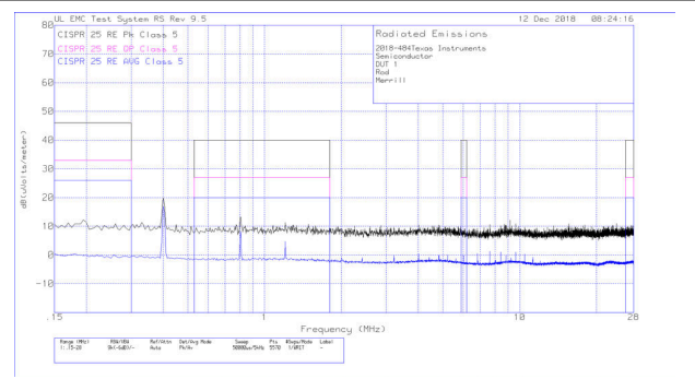
Figure 8-34. Radiated EMI Rod Antenna
