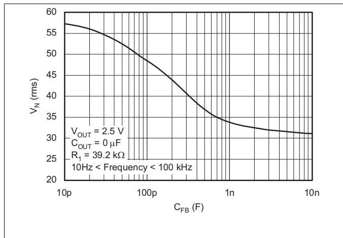
Figure 25. TPS73201 RMS Noise Voltage vs C_{FB}
